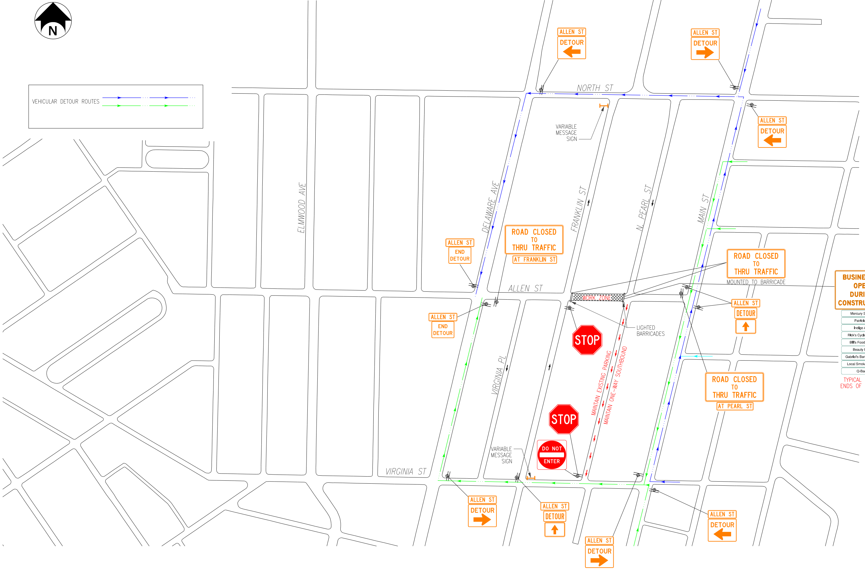
PHASE 2 - STAGE 1 DETOUR PLAN
