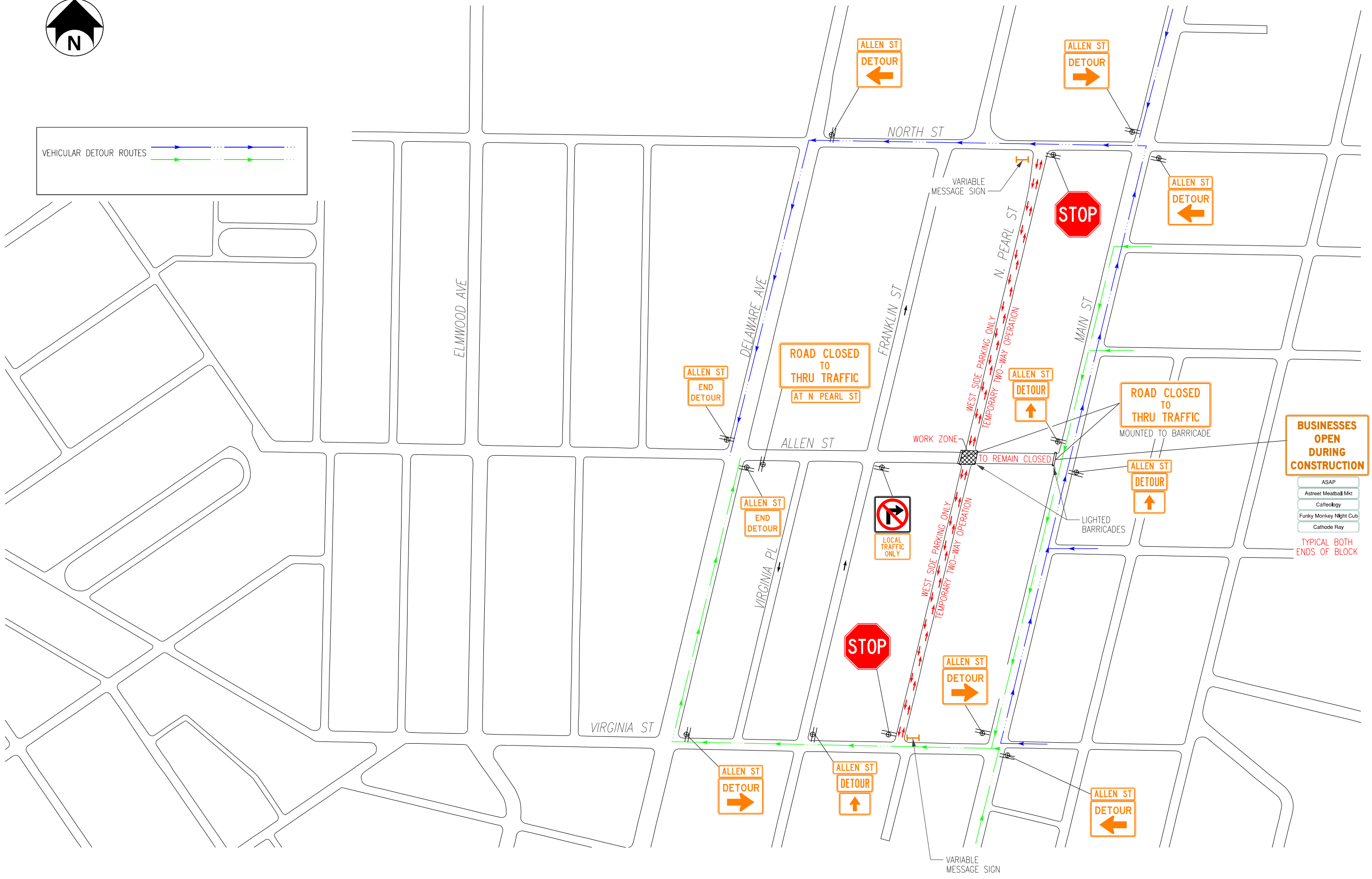
PHASE 1 - STAGE 2 DETOUR PLAN (DURING SHORT-TERM FULL INTERSECTION CLOSURE)
