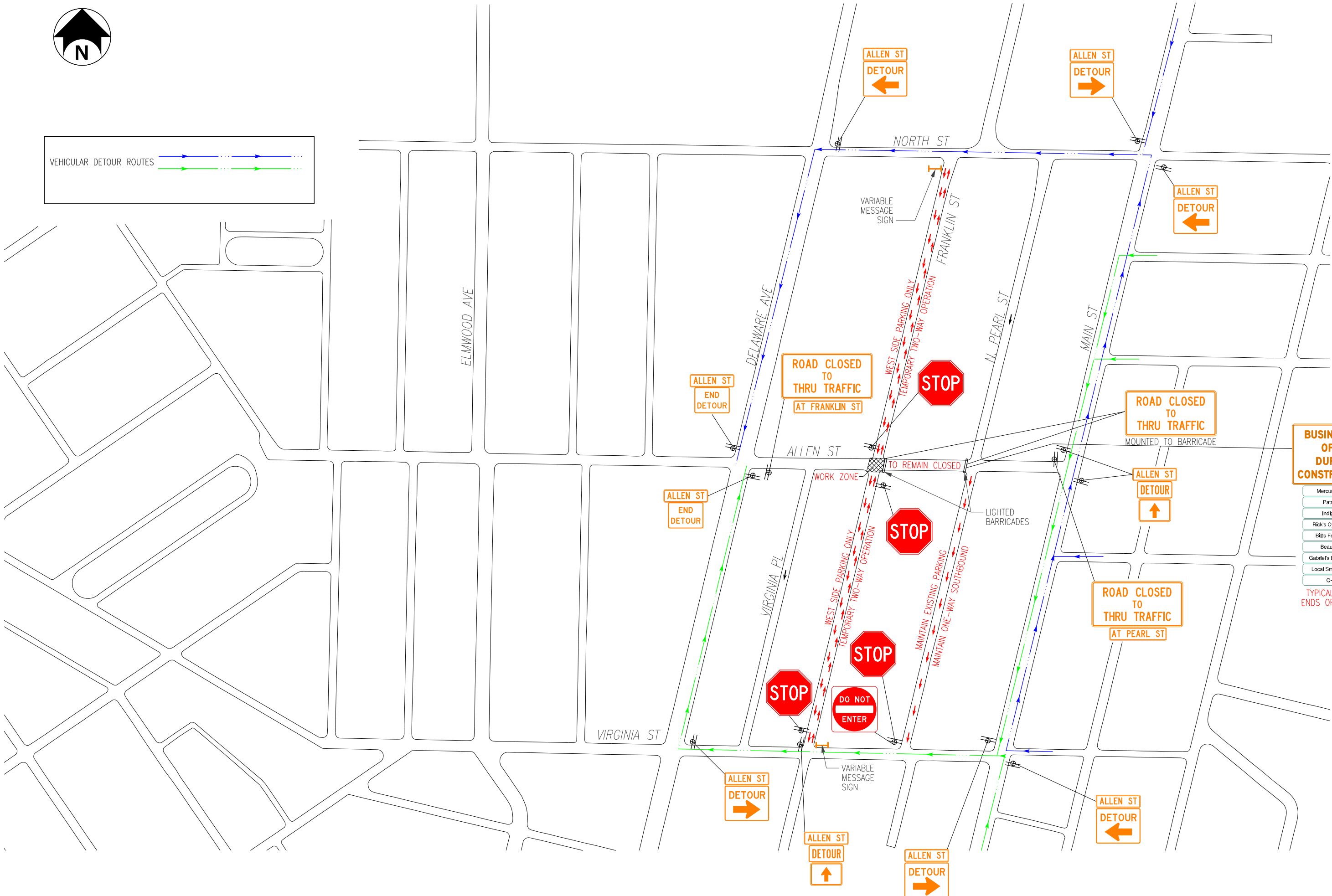
PHASE 2 - STAGE 2 DETOUR PLAN (DURING SHORT-TERM FULL INTERSECTION CLOSURE)
