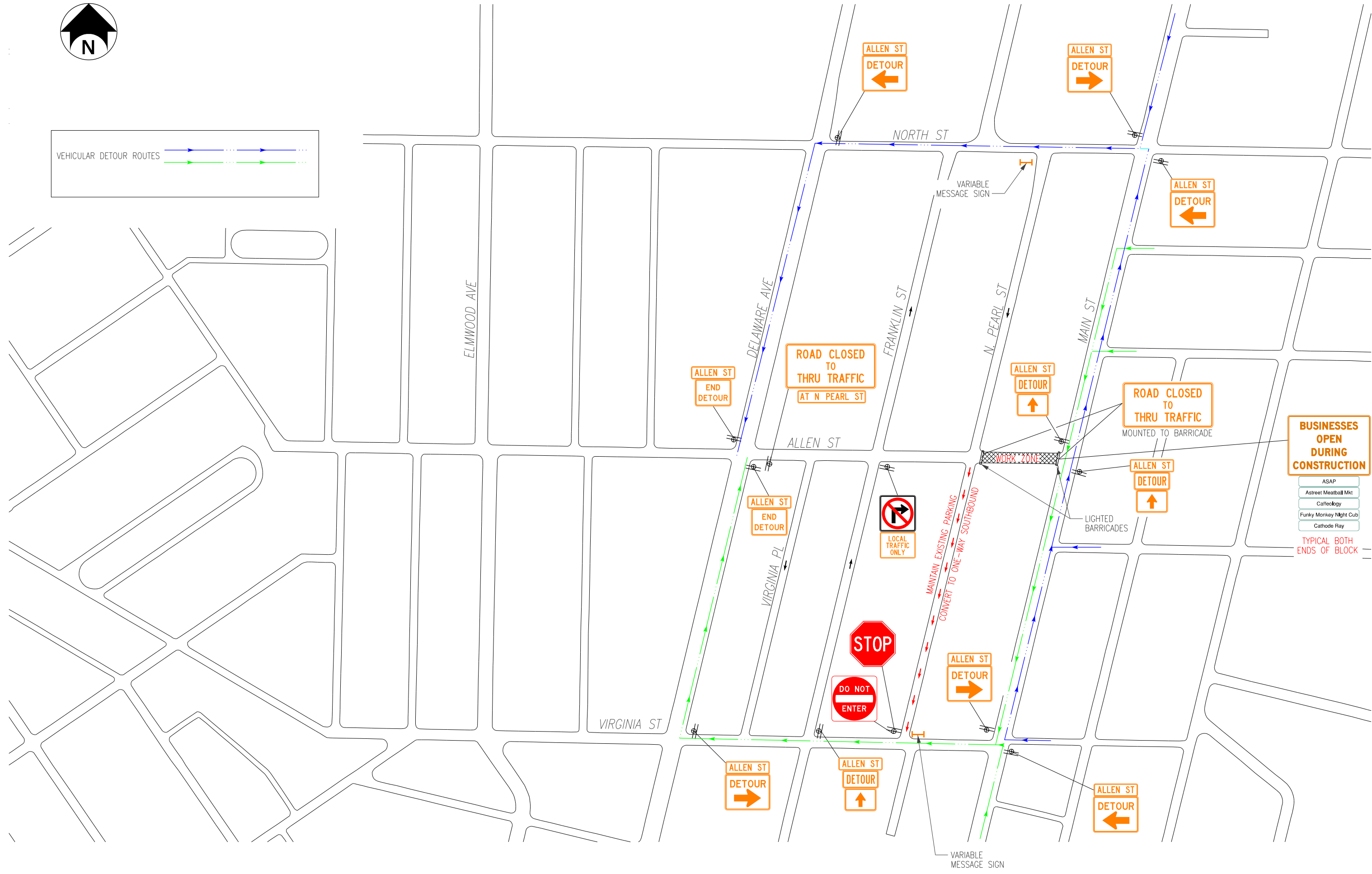
PHASE 1 - STAGE 1 DETOUR PLAN
