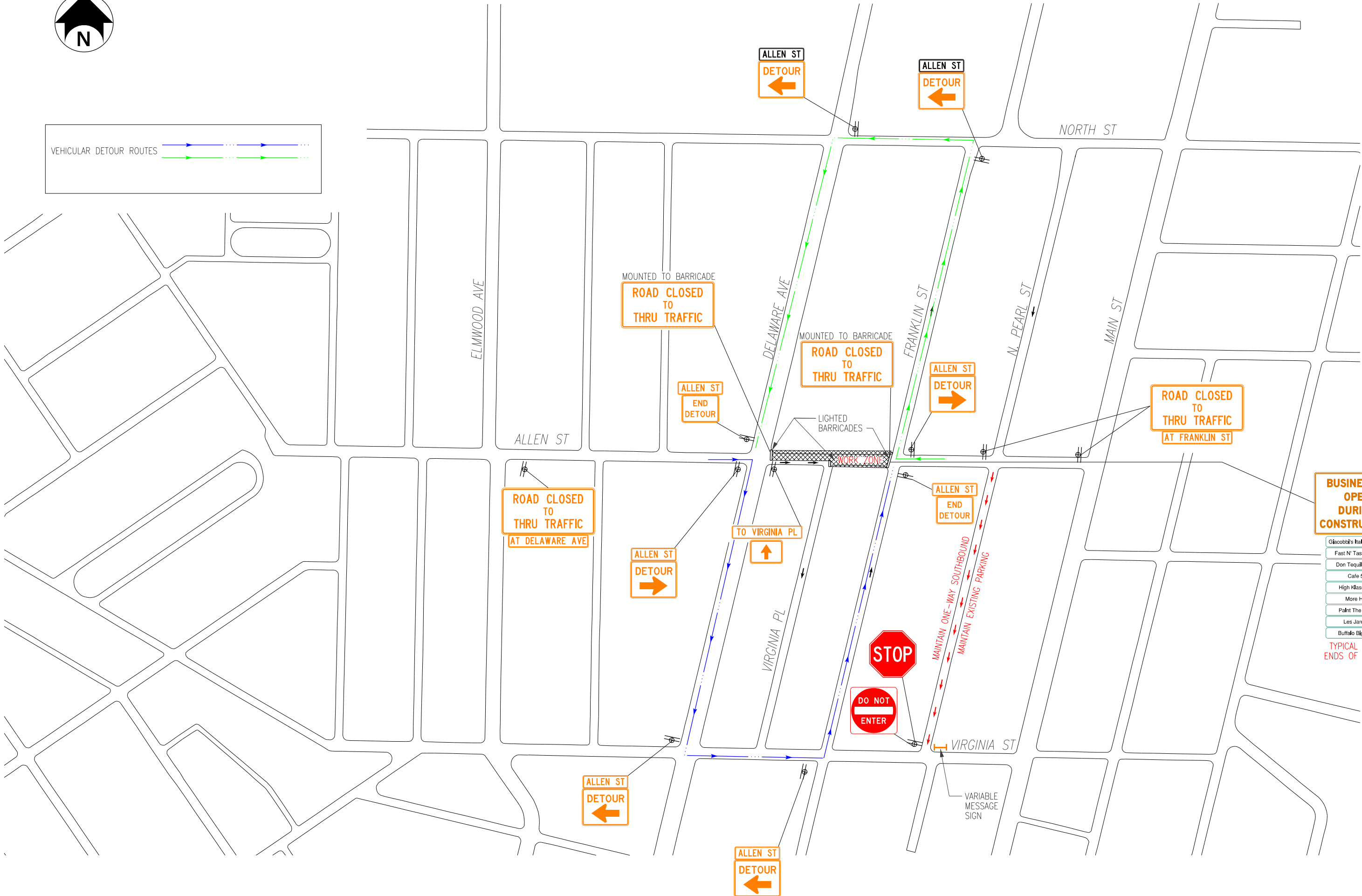
PHASE 3 - STAGE 1 DETOUR PLAN
